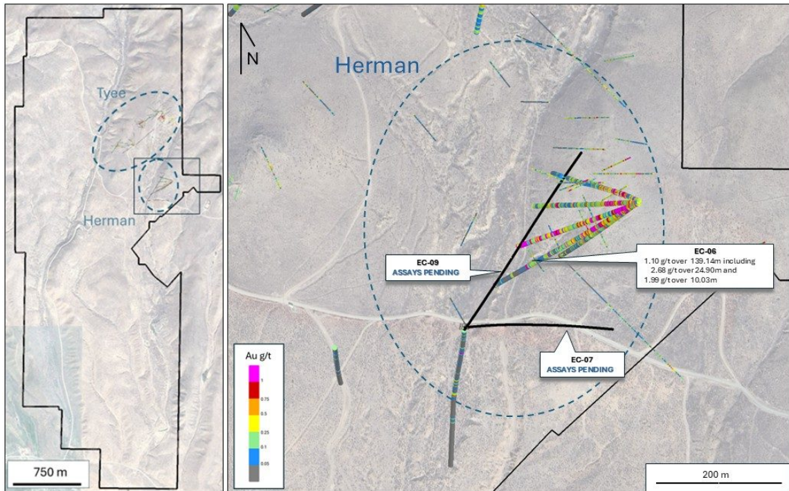
Figure 1. Plan Map of the Herman Drill Locations
